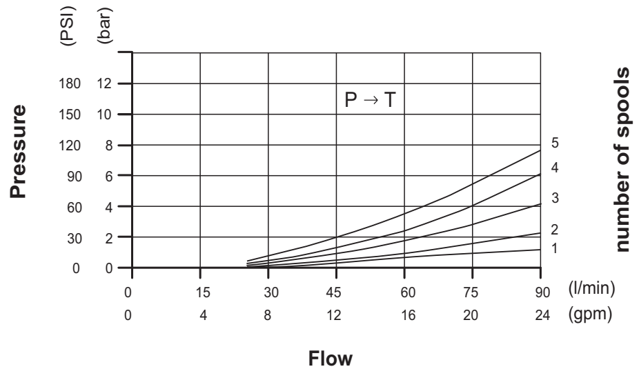
Pressure drop "P" to "T"
