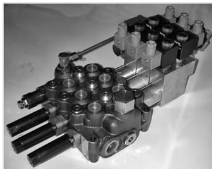
VDM8 - 3 working sections with electro-hydraulic controls H1/H2 - H3/H4
