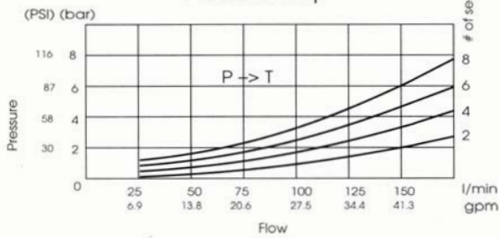
Pressure drop
