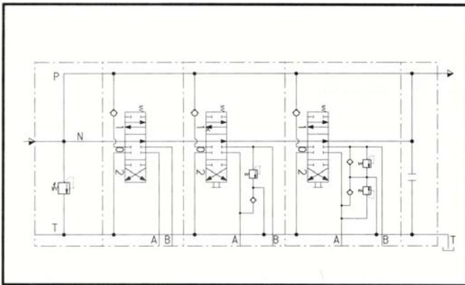
Parallel circuit
