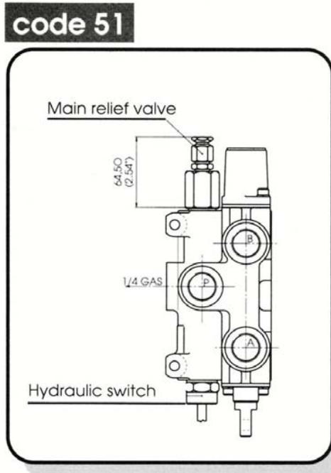
Inlet with hydraulic switch
