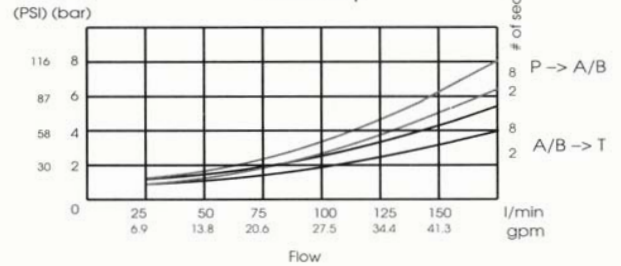
Pressure drop
