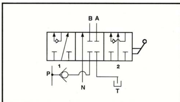
Double acting spool for serie circuit
