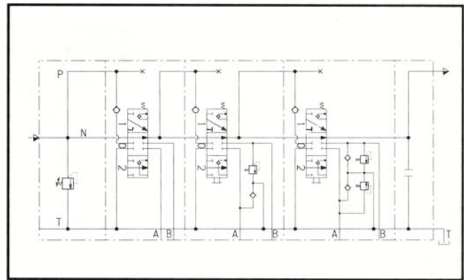
Series circuit
