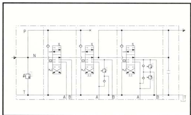
Mixed circuit
