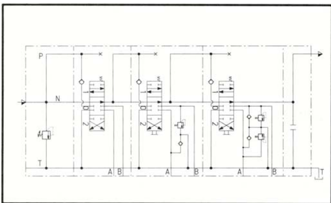
Tandem circuit
