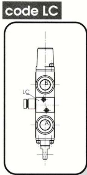
Working section with compensated flow limiting valve
