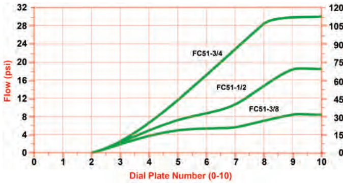
Controlled Flow vs. Dial Plate for FC Series
